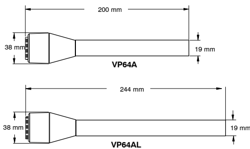
OVERALL DIMENSIONS
